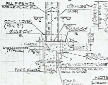
SECTION "1-1" SCALE 3/8" = 1'-0"
