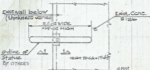
PLAN SCALE 1/8" = 1'-0"
